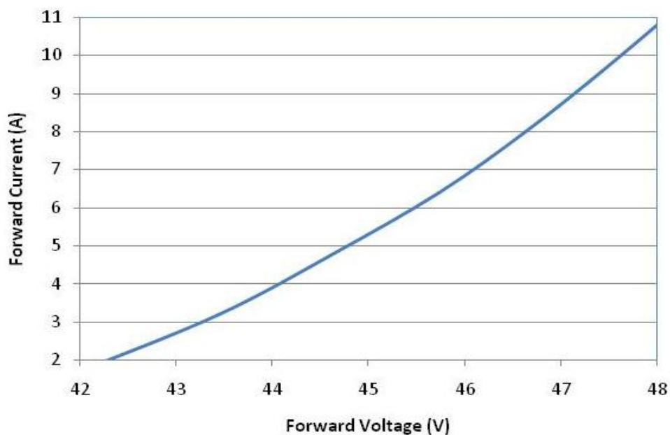
(i) Typical Forward Current (I F ) vs. Forward Voltage (V F ) of Red Section
