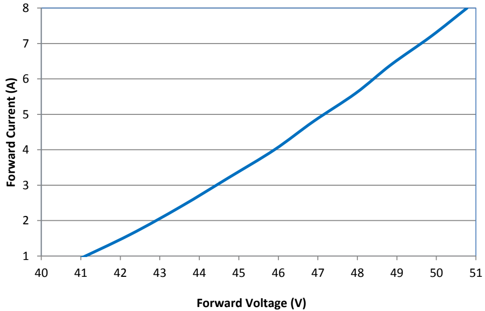
(i) Typical Forward Current ( I_F ) vs. Forward Voltage ( V_F )
